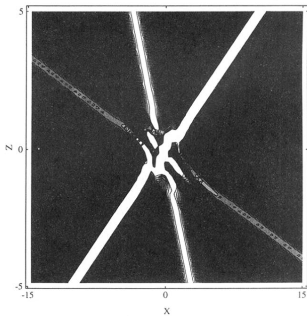
FIG. 1. The refractive index profile of a three-soliton collision. This profile may be considered as a six-port linear device, with three inputs at the bottom of the figure and three outputs at the top.
