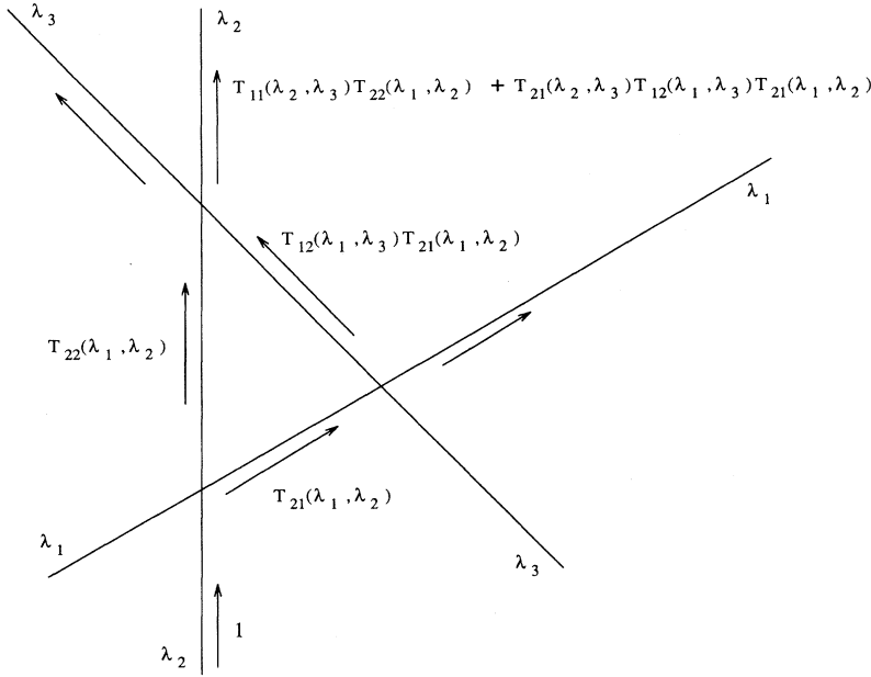
FIG. 3. Calculation of the N=3 matrix element T_{22} from the N=2 matrix elements.
