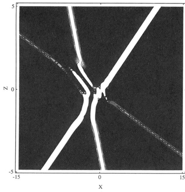
FIG. 2. The refractive index profile of a three-soliton collision. This waveguide has the same transmission properties as that shown in Fig. 1.
