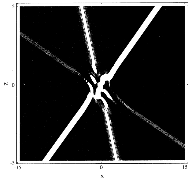
FIG. 1. The refractive index profile of a three-soliton collision. This profile may be considered as a six-port linear device, with three inputs at the bottom of the figure and three outputs at the top.
